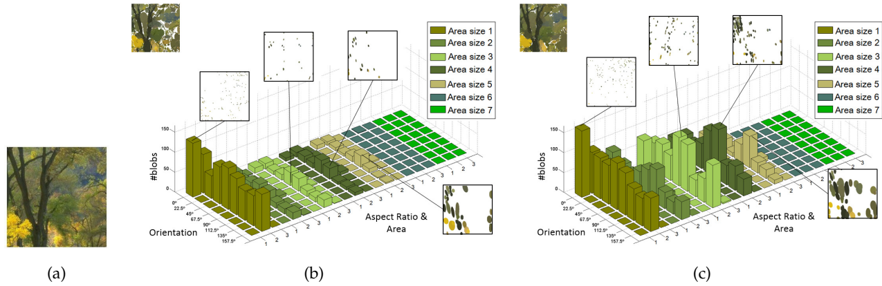
Fig. 7. Comparison of the shape descriptors of an image (a) obtained on the opponent space (b) and on the MTT representation (c). Shape descriptors are shown as a 3D histogram where each bin clusters detected blobs with similar area, orientation and aspect ratio. On the aspect ratio and area axis, '1' corresponds to isotropic blobs, '2' to elliptical blobs, and '3' to highly-elongated blobs. Bins corresponding to different areas are plotted in different colors. Area increases along the axis.
