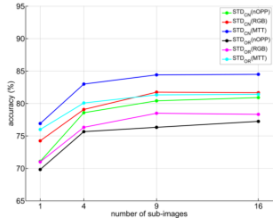
Fig. 8. Accuracy on scene recognition in terms of the number of sub-images used to compute STD descriptors on different color spaces.
